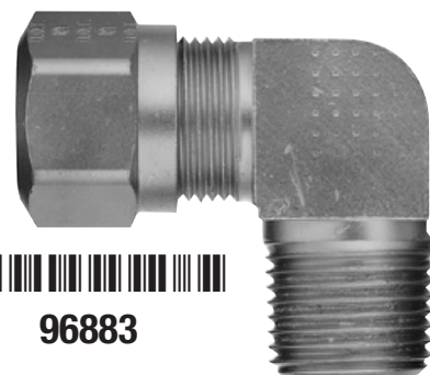
Male Elbow 90° 3/4 Tube x 1/2 NPT
